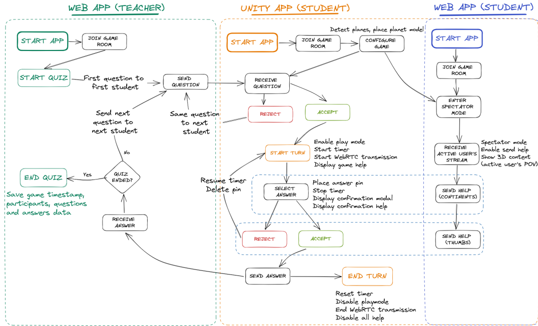
Figure 4.1: Workflow of the AAroundTheWorld application.
